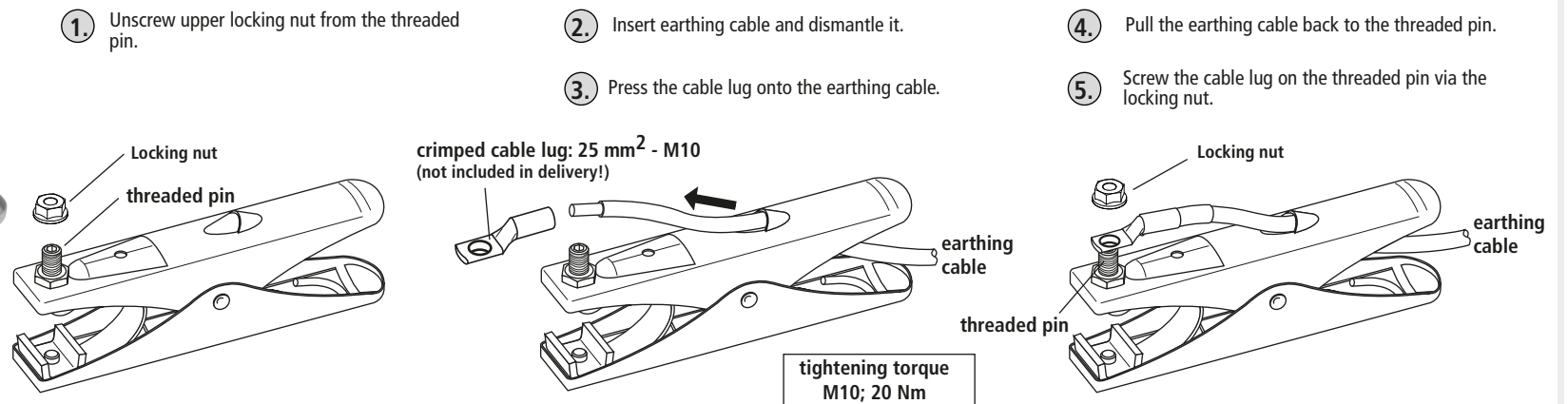
Fig. 2 Connection
