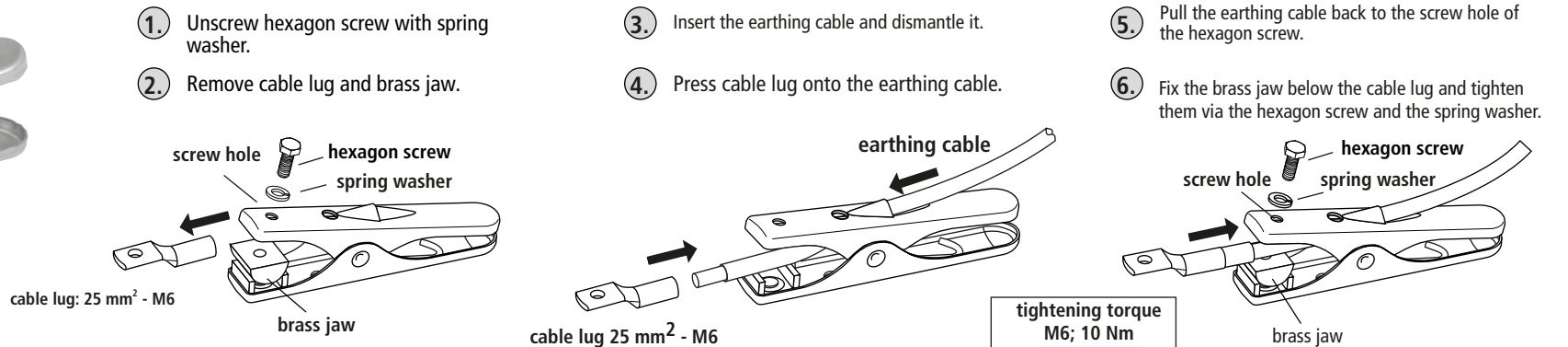
Fig. 2 Connection
