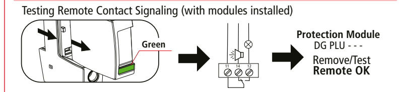
Fault Indication
