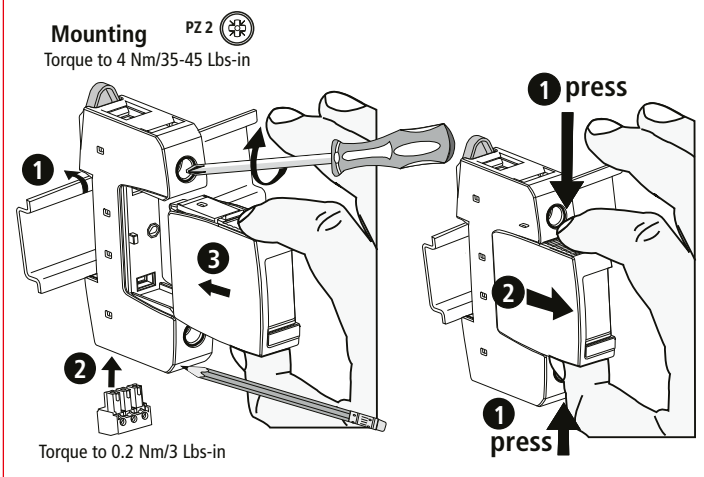
Mounting
