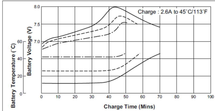
Charge Characteristics (5 cells pack)
