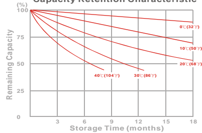
Capacity Retention Characteristic
