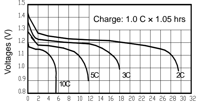
Discharge characteristics
