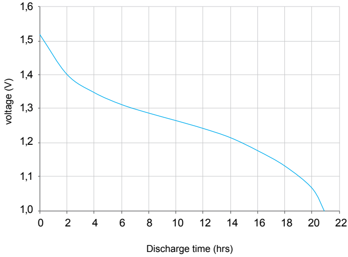
Remote Control 15s/m 8h/d 24 ohm cutoff 1,0 V
