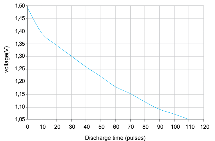
Digital still Camera 10x(2s 1,5W/28s0,65W)5m,55m off 24h/d cutoff 1,05 V
