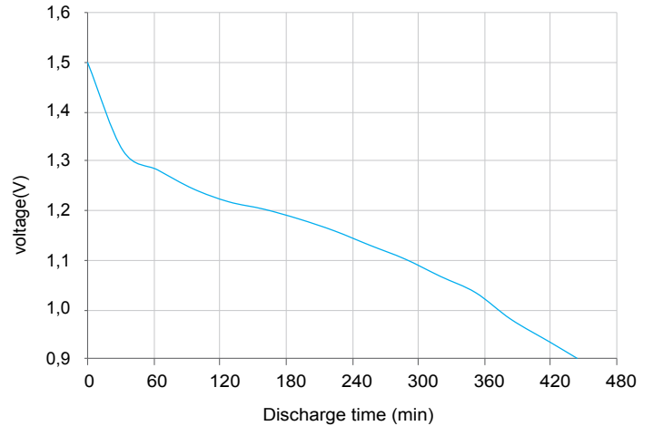
Portable lighting (LED) 4m/h 8h/d 3,9 ohm cutoff 0,9 V
