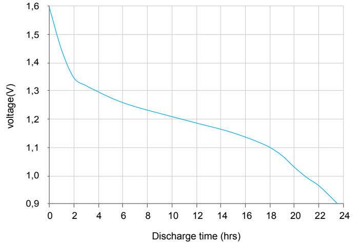
CD, digital audio, wireless gaming and accessories 1h/d 100 mA cutoff 0,9 V
