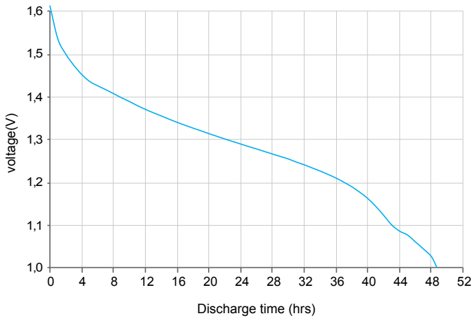
Radio/ Clock / Remote Control 1h/8h 50 mA cutoff 1,0 V
