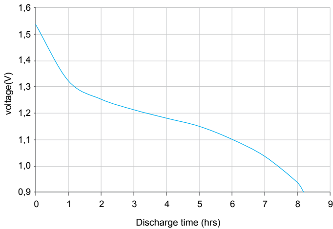
Toy, non-motorized 1h/d 250 mA cutoff 0,9 V
