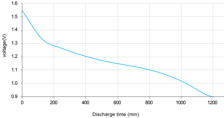
Portable Lighting 4m/15m 8h/d 3,9 ohm cutoff 0,9V
