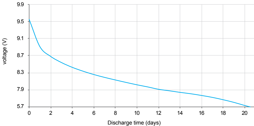
Smoke detector 10 kohm 24h/d + 620 ohm 1s/h cutoff 7,5 V
