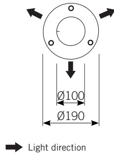
Accessory Flange
