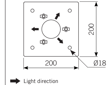
Accessory Plate
