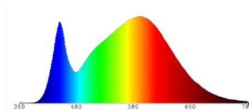
CCT - 4000K
