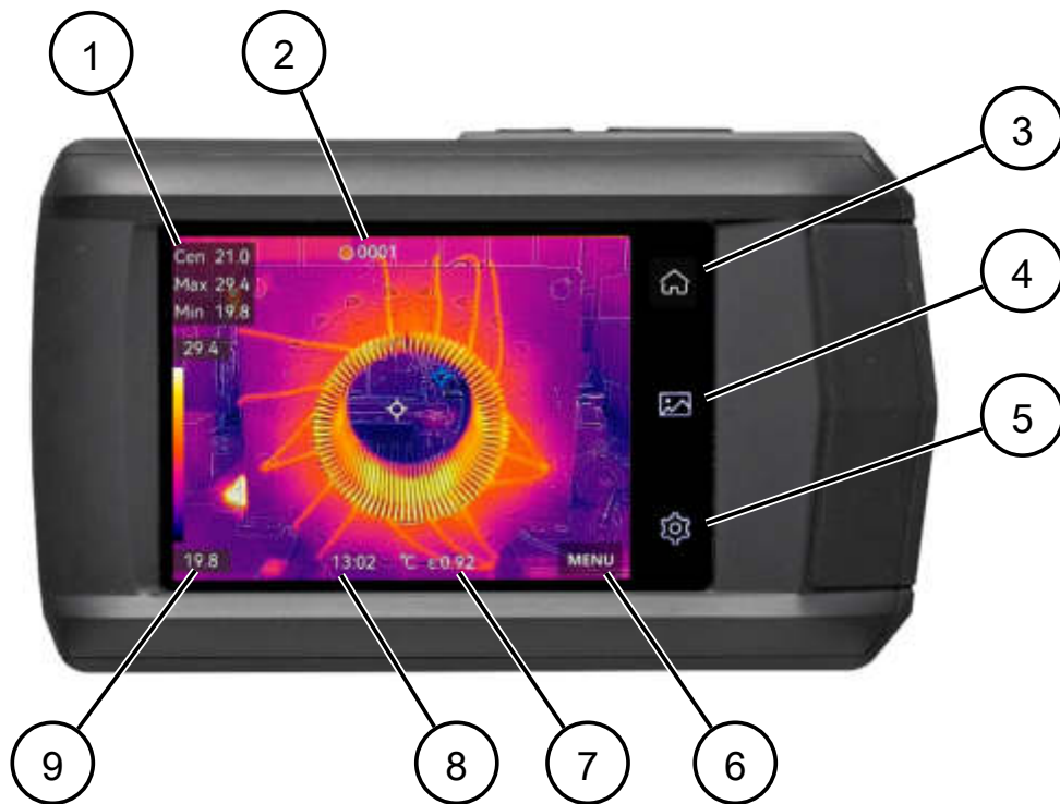
Figure 2: Touch display
