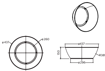
91401812987 Highbay Reflector AL-L_Z
