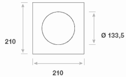
Lochblende SQ-DLA1-M
