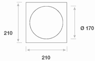
Lochblende SQ-DLA1-L
