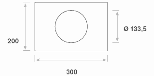
Lochblende RCT-DLA1-M
