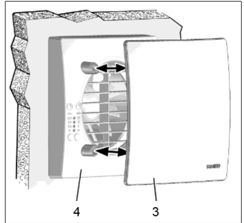
3 Designer cover
