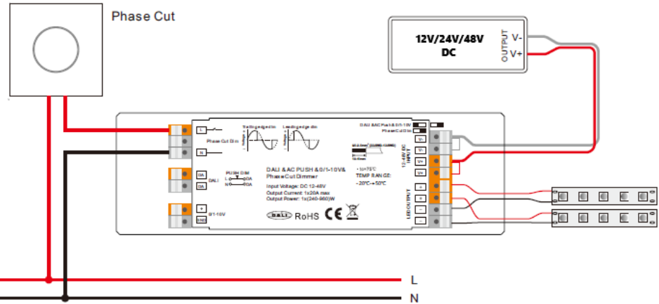
Abb. 05 - Phasendimmung
