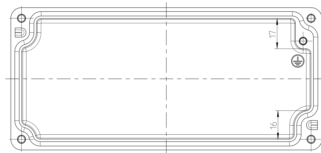
Innenansicht Deckel/ interior view lid
