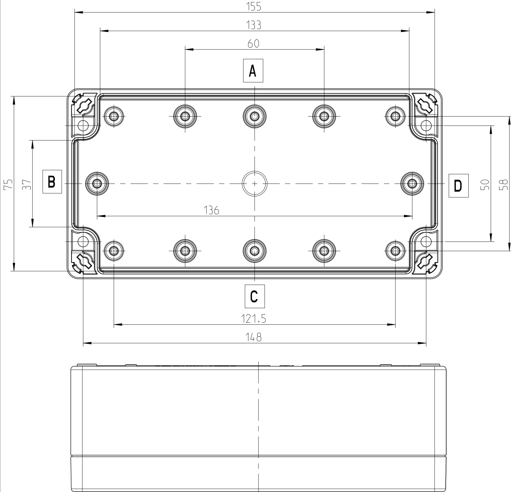
Innenansicht/interior view
