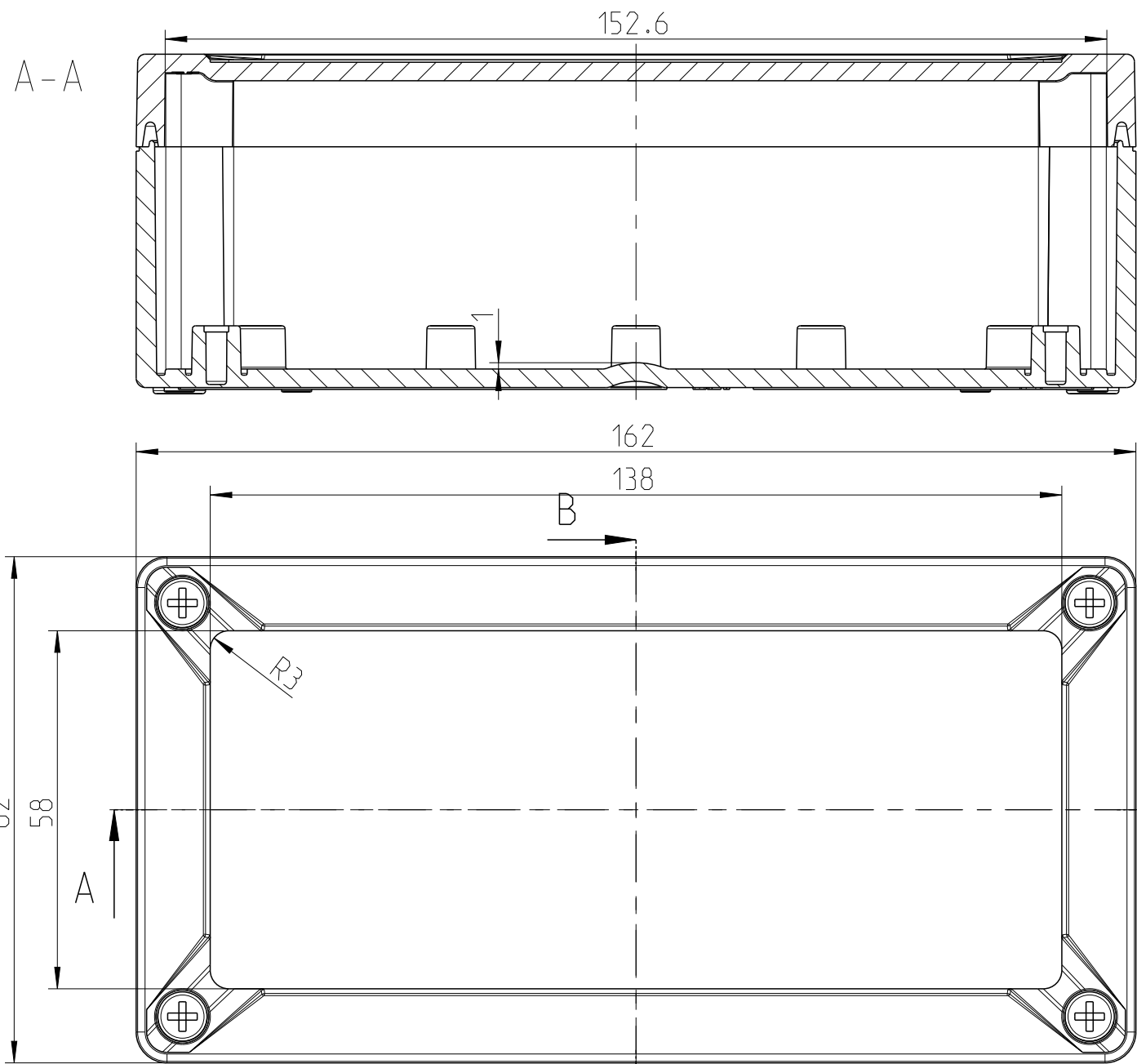
Innenansicht/interior view
