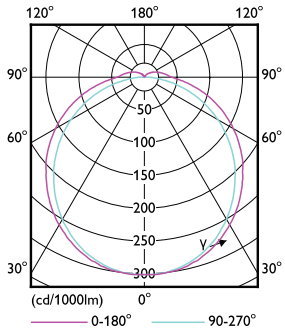
Light Distribution Diagram - CorePro LED PLT HF/Mains 6.5W 830 4P
