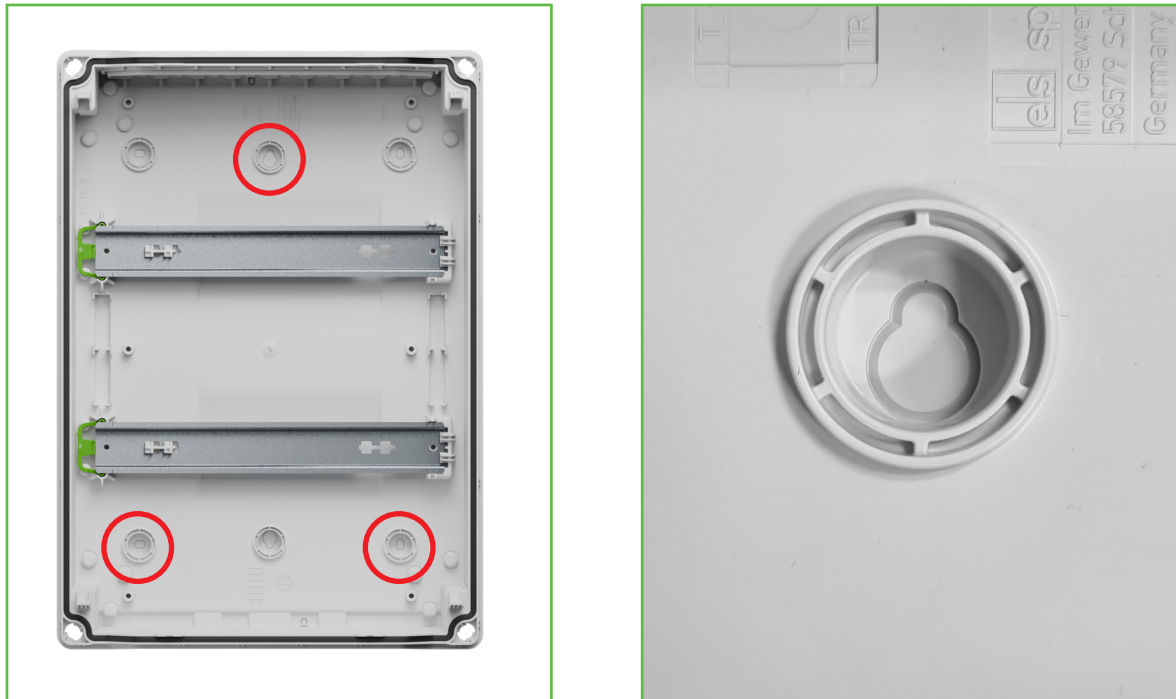
Figure 23: Fastening points 3-point installation, keyhole fastening
