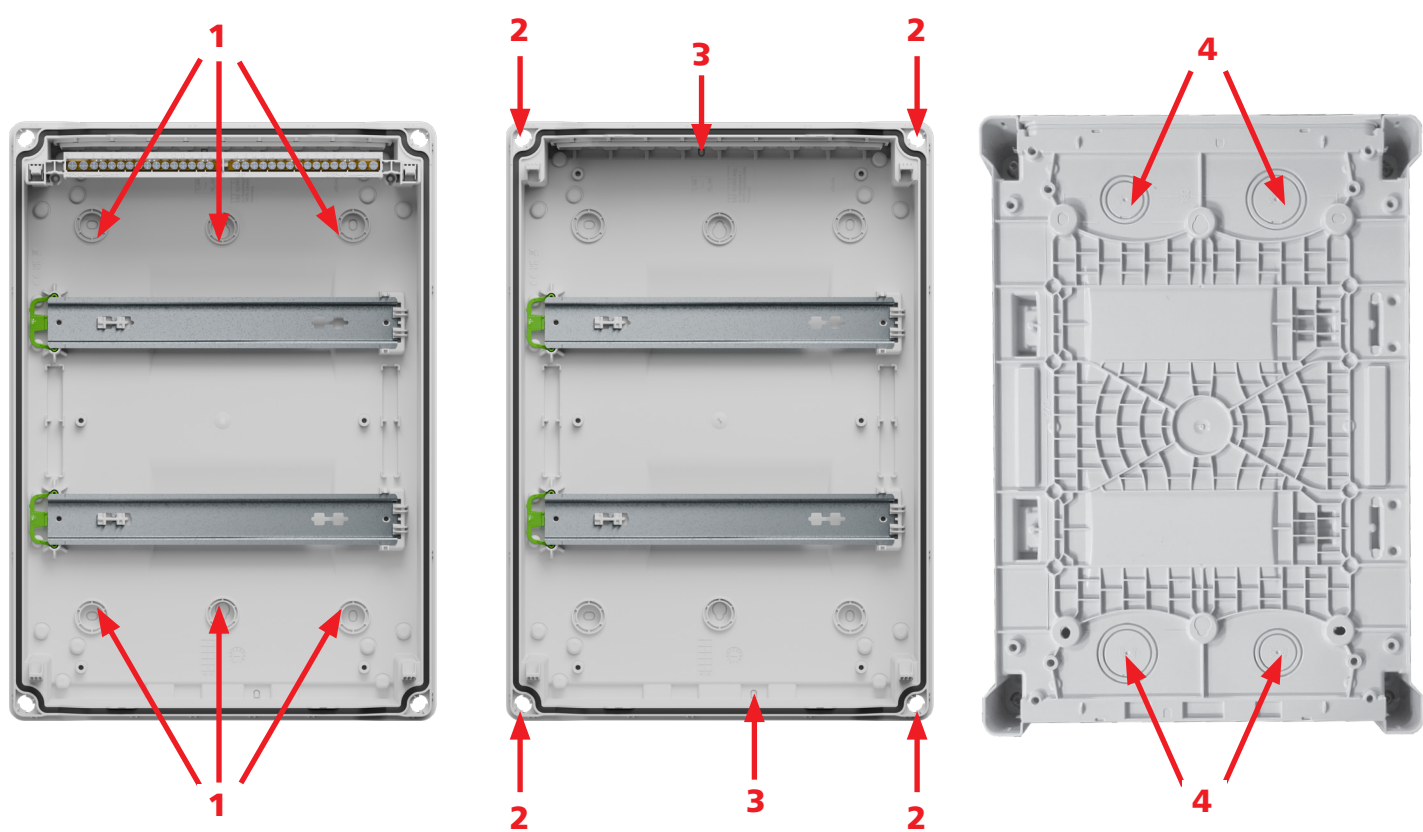
Figure 2: Box bottom front side, back side
