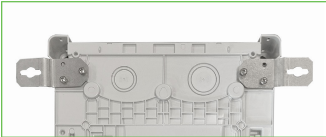
Figure 20: Fixing points external lugs
