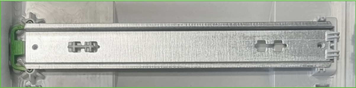
Figure 7: Standard rail on standard rail holder
