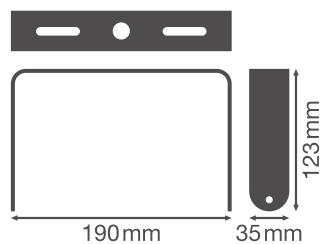
HB COMP BRACKET 120W
