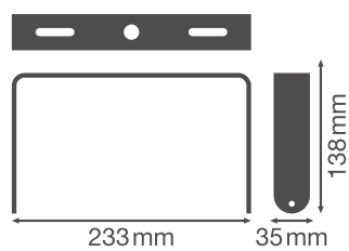
HB COMP BRACKET 220W
