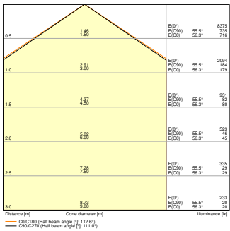
PL COMP 1200X600 DA V 44W 840 5880lm
