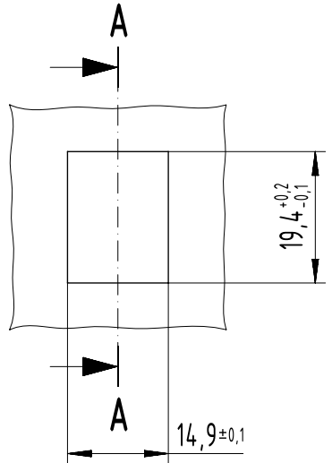
Panel cut out (1:1)
