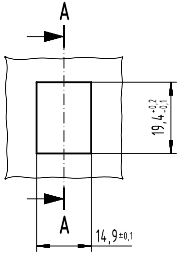
Panel cut out (1:1)
