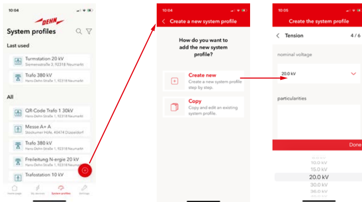
Figure 10 Create new system profile
