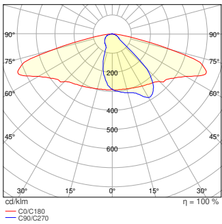
UFLEXS6P060W 740RV35ST 2 NC0UGC240X
