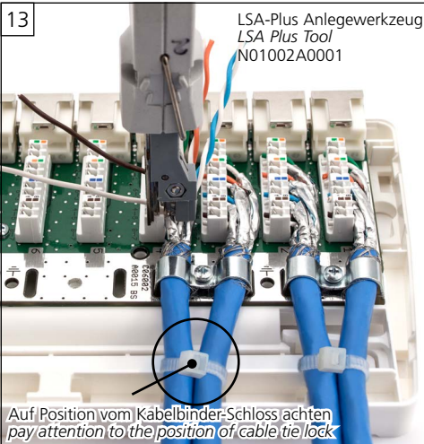
AMJ- / UMJ-Module und Kupplungen AMJ- / UMJ Modules and Couplers
