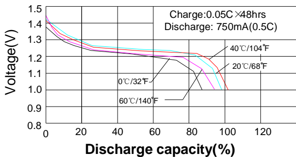
Discharge characteristics
