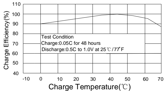
Charge efficiency
