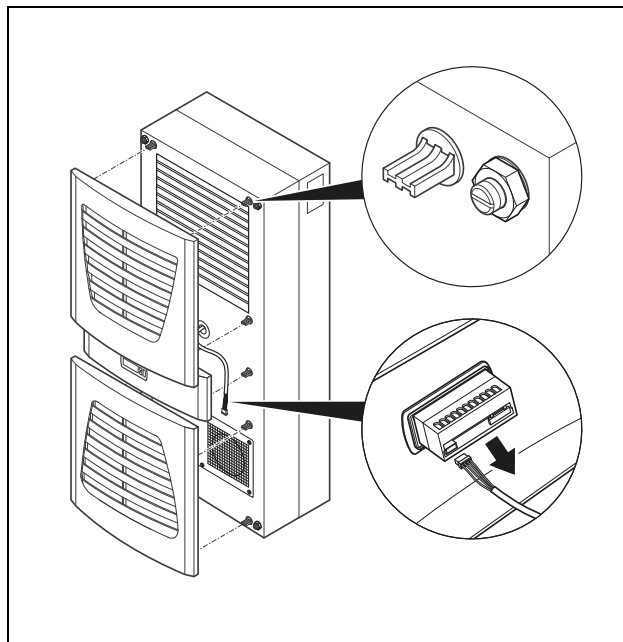
Fig. 15: Remover a grade e desligar o display
