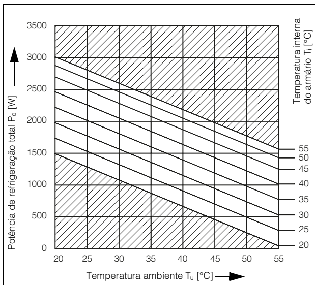
Fig. 109: 3366.xxx (plano), 1500 W, 400 V/50 Hz
