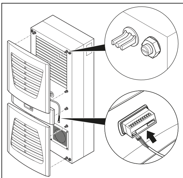
Fig. 32: Conectar o display e colocar as grades
