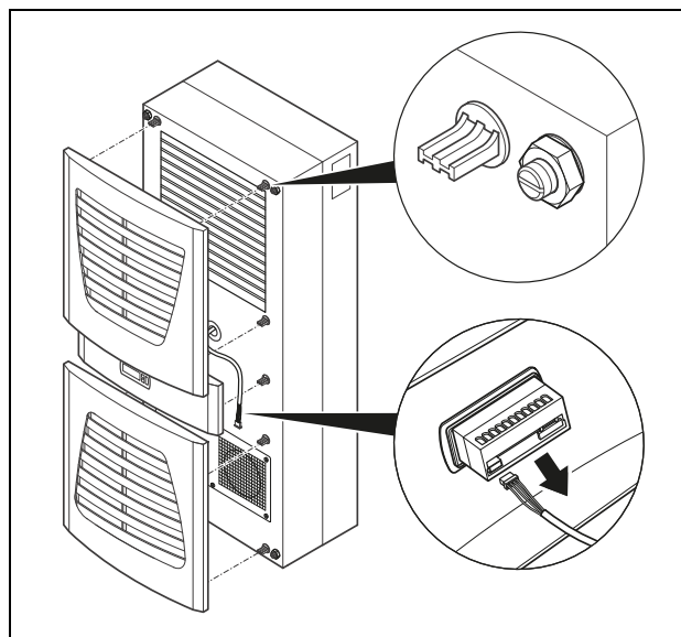
Fig. 10: Remover a grade e desligar o display
