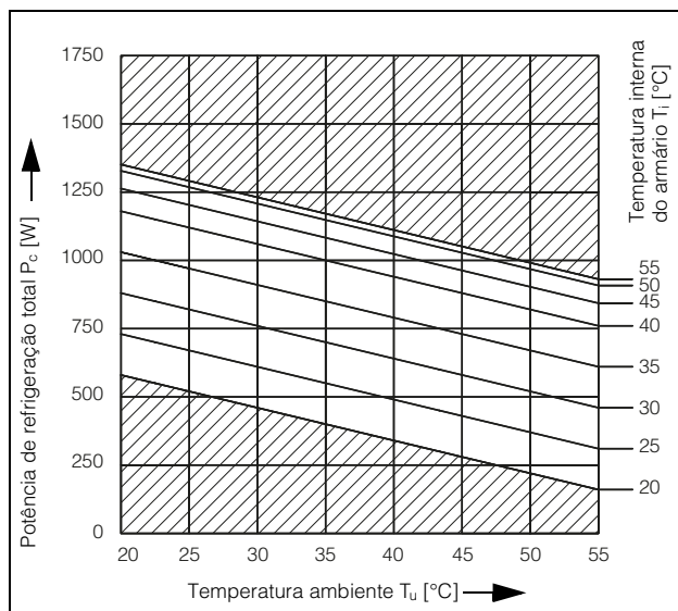
Fig. 93: 3361.xxx, 750 W, 50 Hz
