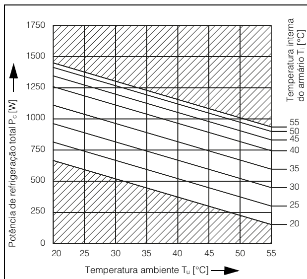
Fig. 94: 3361.xxx, 750 W, 60 Hz
