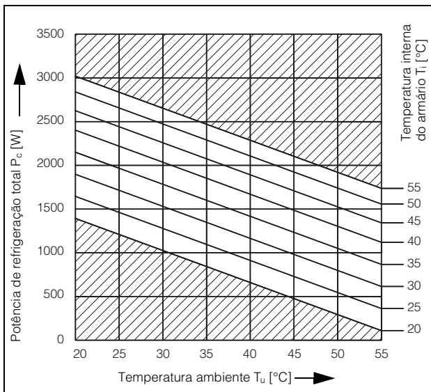
Fig. 99: 3366.xxx (plano), 1500 W, 50 Hz
