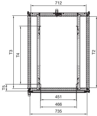
Kesit A – A, IP 55
