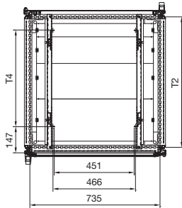
Kesit A – A, IP 55
