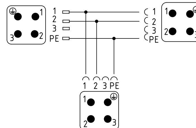
wiring diagram
