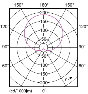
CorePro LEDbulb ND 10-75W A60
