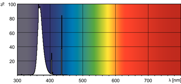
Spectral Power Distribution Colour - TL 60W/10-R SLV/25
