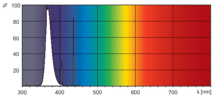
Spectral Power Distribution Colour - Actinic BL TL-D 15W/10 Secura 15L/25
