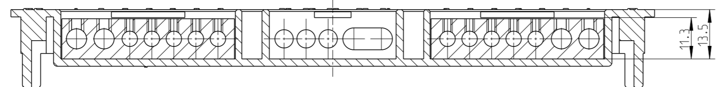
A-A Innenansicht/ interior view
