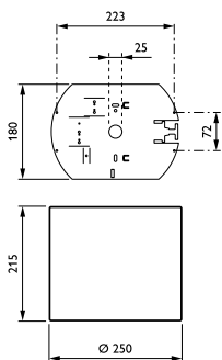
DN570C LED24S/840 PSU-E C WH
