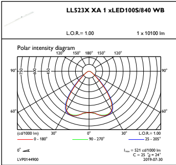
OFFPC1_LL523XXA1xLED100S840WB
