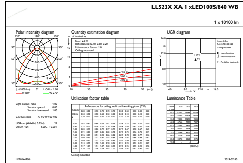
IFGU1_LL523XXA1xLED100S840WB
