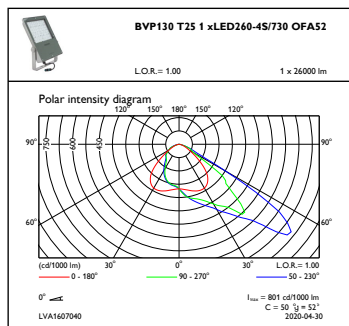
OFPC1_BVP130T251xLED260-4S730OFA52
