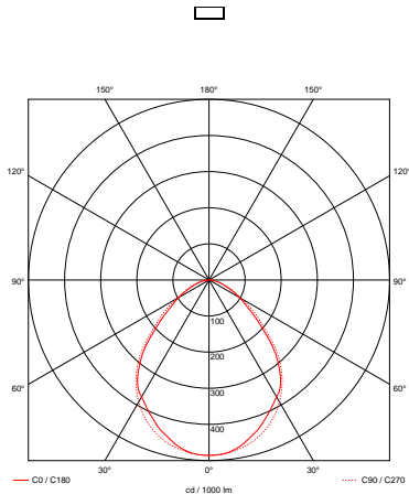
LightE@ PRACHT_BERNINA_F_Idt_1x32W_breit90_1274mm.Idt. Light Diagram
