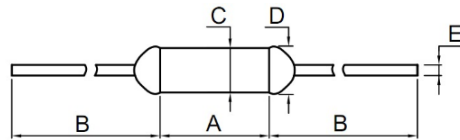
Dimensions (mm)
