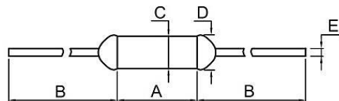
Dimensions (mm)
