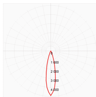
TLM1-24°
